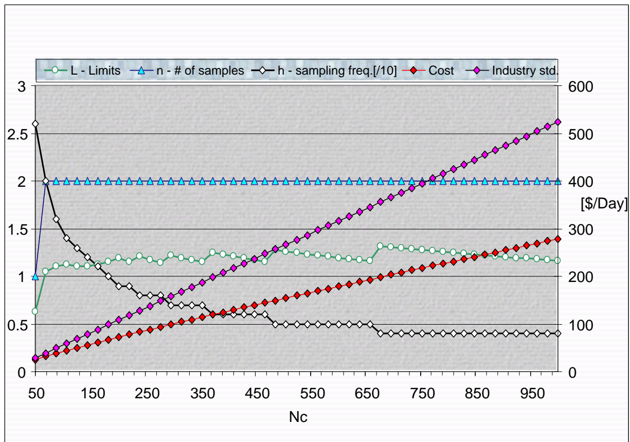
Figure 4. Effect of number of cows in the herd ( N_c ) on optimal sampling design and total quality costs per day; L = the optimal control limits for an X-bar chart, n = the number of samples to be taken at each sampling time, and h = the sampling frequency expressed in days/10. The cost is the total quality cost per day. The industry standard curve is the total quality cost for the herd if a conventional sampling design is used (i.e., n = 1 , h = 30 d, and L = 2 ). Note that for a herd of 1000 cows (becoming increasingly more frequent in the USA) the economic return to using an optimal sampling design (bottom diamond line) vs. the conventional design (upper diamond line) exceeds 250 US$/d.
